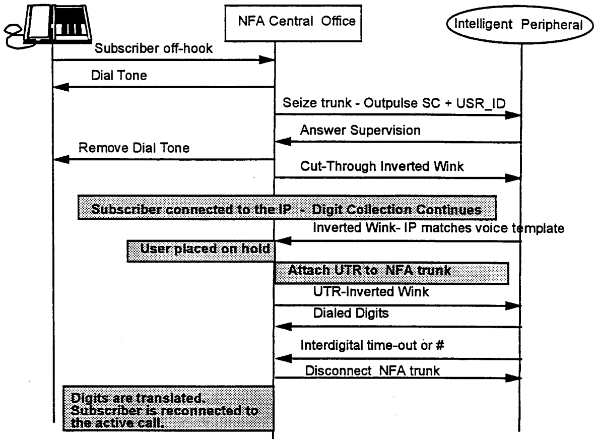
Figure 2 - Implicit Connection, IP Dials the Call
